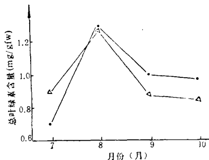
图2 1989年废黄河口互花米草叶绿素含量 “△”表示A含量, “•”表示B含量。 Fig.2 Chlorophyll contents of S.alterniflora near the estuary of old yellow river in 1989. note: “△” means the content of community A, and “•” is that of B.
